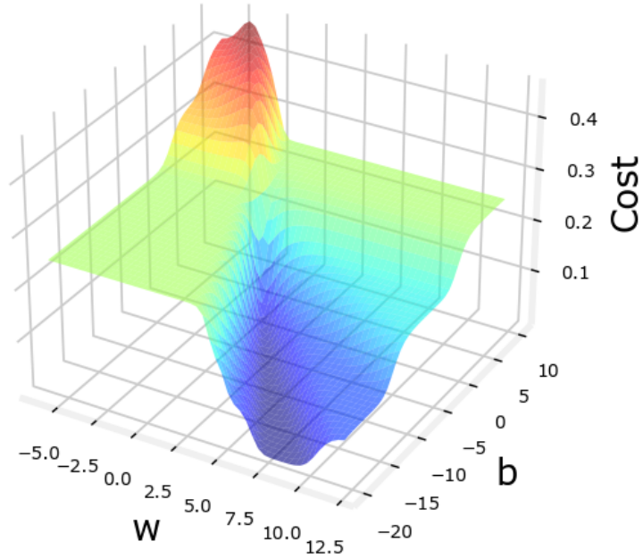
"Logistic" Squared Error Cost vs (w, b)
