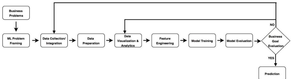
Figure 1 – End-to-End Machine Learning Process
