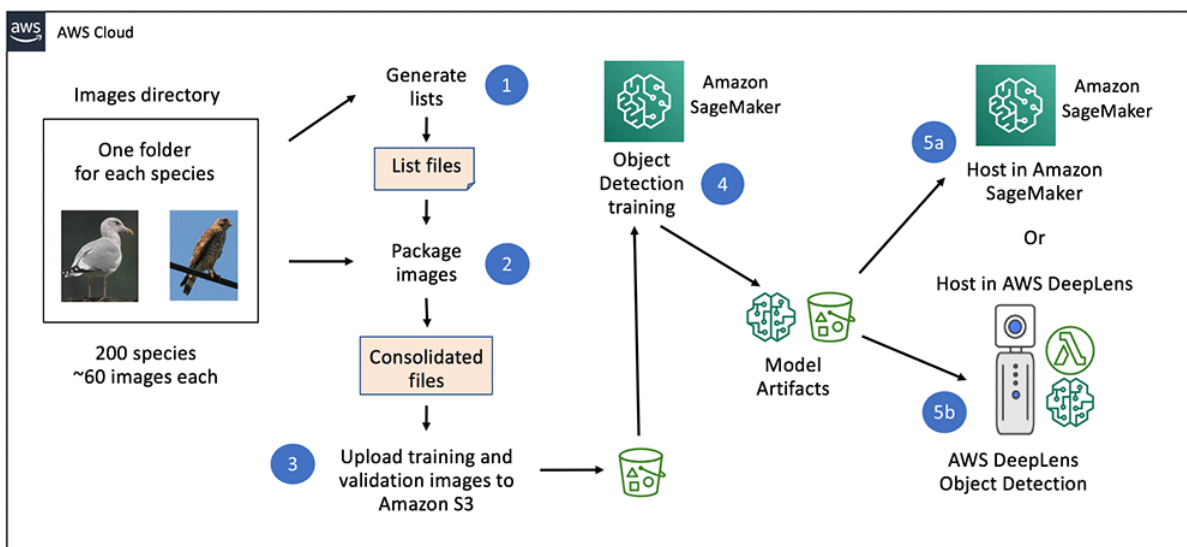
Figure 7 – Bird Species Identification on the Edge Architecture
